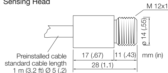
Sensing Head
