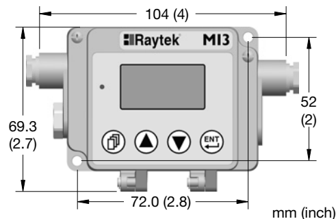
MI3M Multi-channel Electronics Housing
